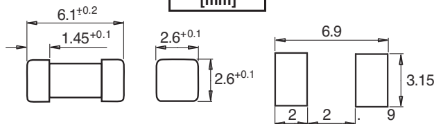
Recommended pad layout
