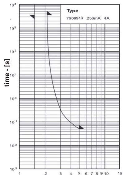
Time-Current Characteristics
