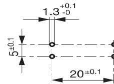
Drill Pattern
