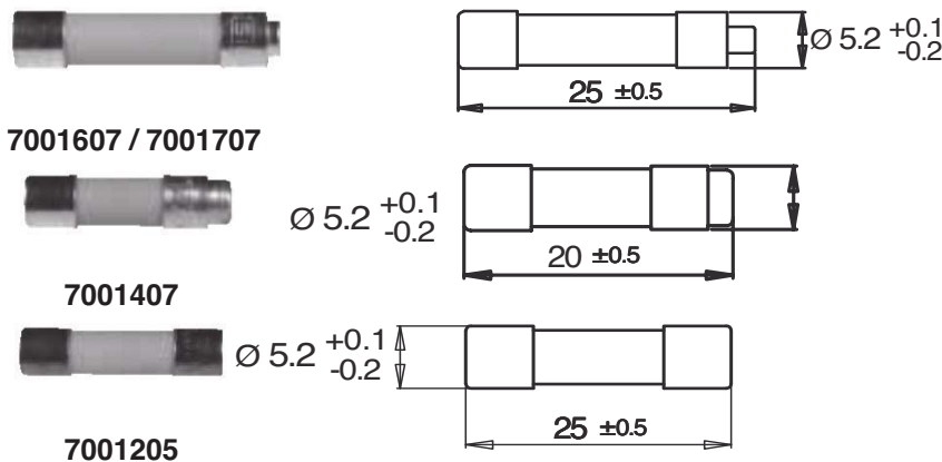
Dimensions [mm]
