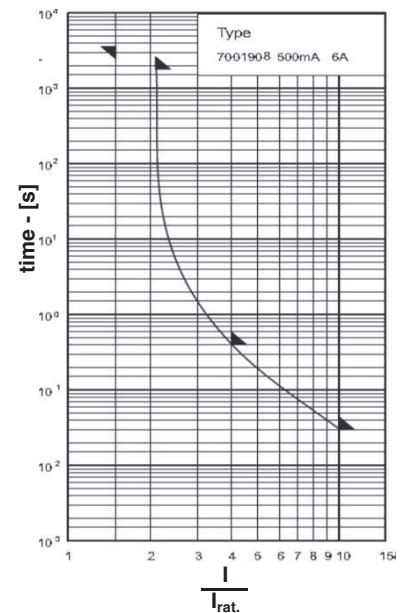
Time-Current Characteristics
