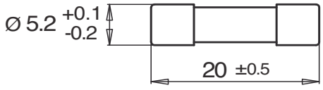
Dimensions [mm]
