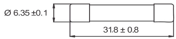
Dimensions [mm]
