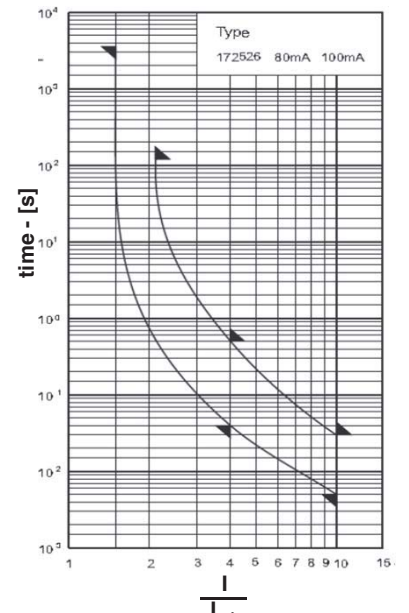
Time-Current Characteristics
