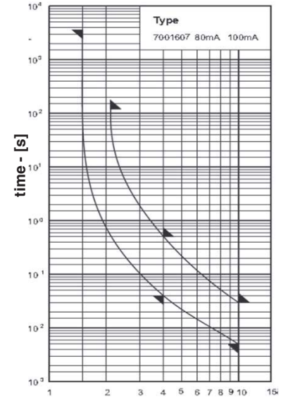
Time-Current Characteristics
