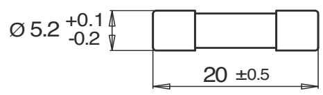
Dimensions [mm]
