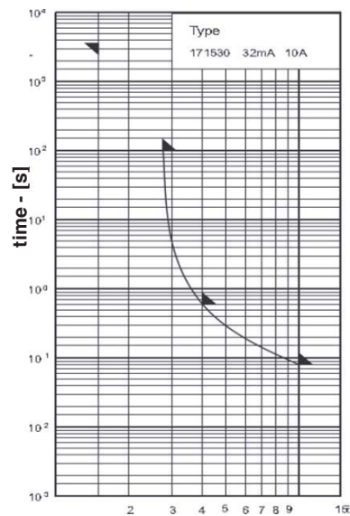
Time-Current Characteristics
