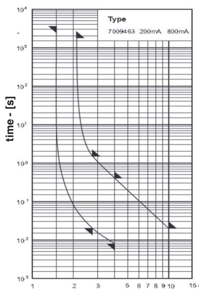
Time-Current Characteristics
